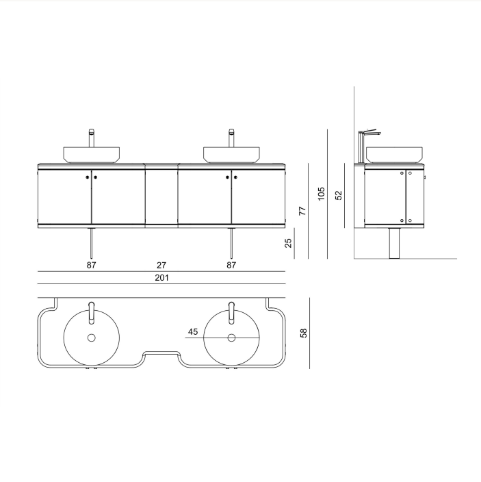
DOIOR1 L 200 x H 90 x W 57 cm
