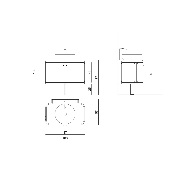
DOIOR2 L 87 x H 90 x W 57 cm
