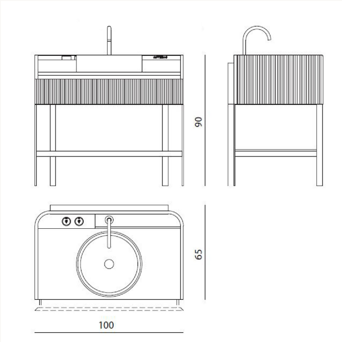
KBOOR2 L 100 x H 90 x W 65 cm
