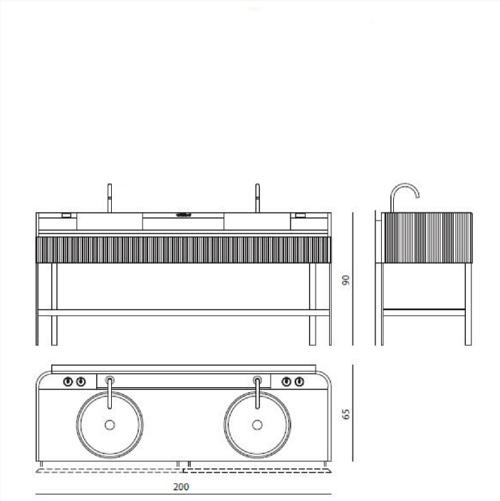
KBOOR1 L 200 x H 90 x W 65 cm
