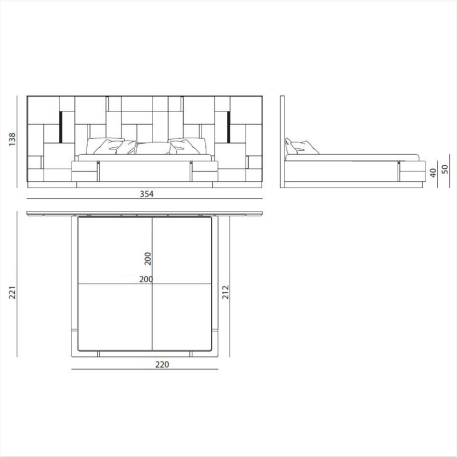
BLVL20 L 354 x H 138 x W 220 cm
