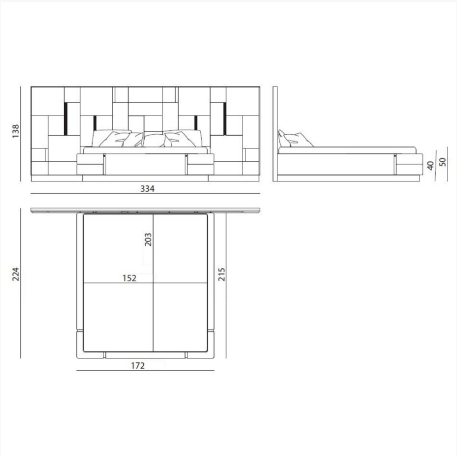
BLV152 L 334 x H 138 x W 223 cm
