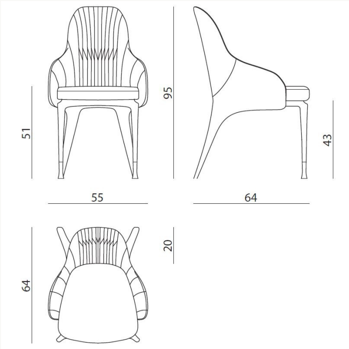
PAYPYA L 55 x H 95 x W 64 cm
