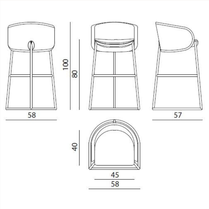
SNI1S0 L 58 x H 100 x W 57 cm
