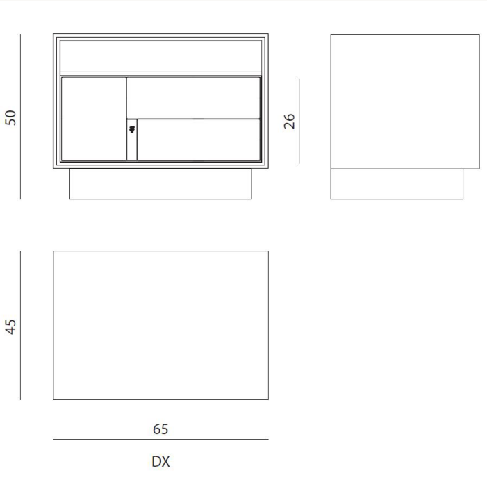
BELDXC L 65 x H 50 x W 45 cm
