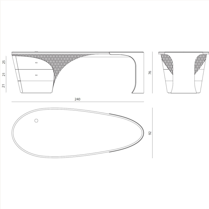
JET JEZ L 240 x H 76 x W 92 cm
