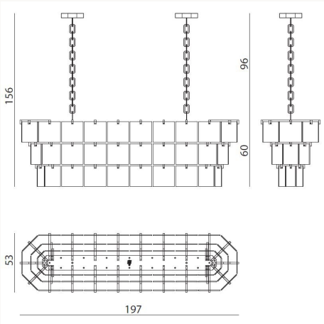
BRNLPQ L 197 x H 60 x W 53 cm
