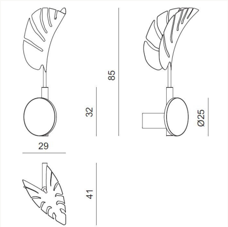
CIABG2 L 29 x H 85 x W 41 cm
