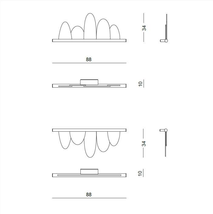
PDEAD2 L 88 x H 34 x W 10 cm
