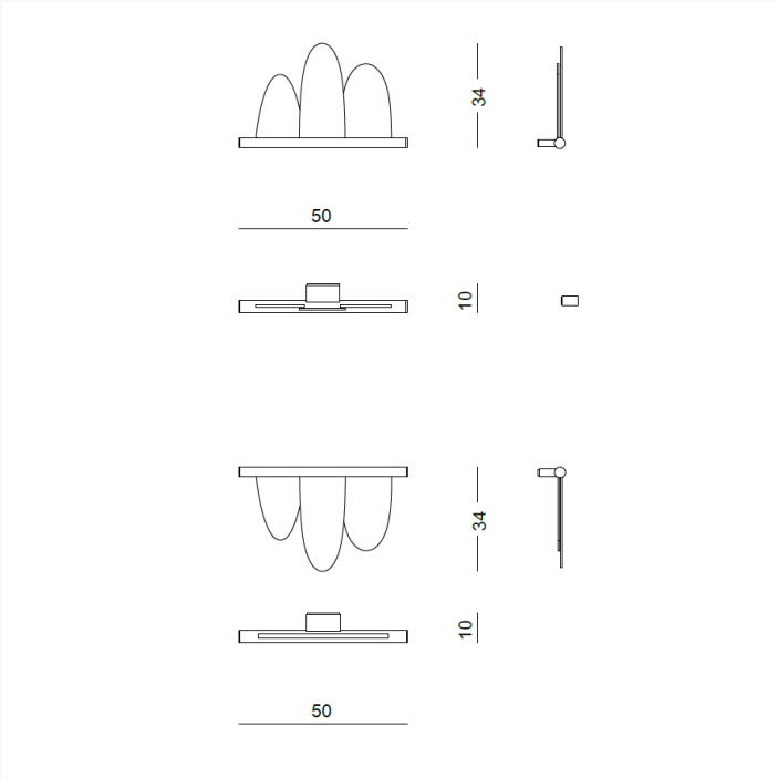
PDEAD3 L 50 x H 34 x W 10 cm
