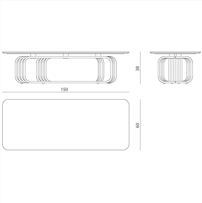
VNCVN1 L 150 x H 38 x W 60 cm
