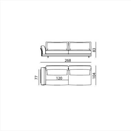
ANHE6S L 268 x H 83 x W104 cm
