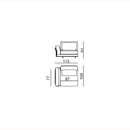
ANHLAS L 115 x H 83 x W 104 cm
