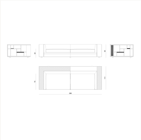
BYRK73 L 298 x H 64 x W 111 cm
