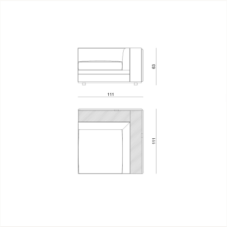
BYRK11 L 111 x H 64 x W 111 cm
