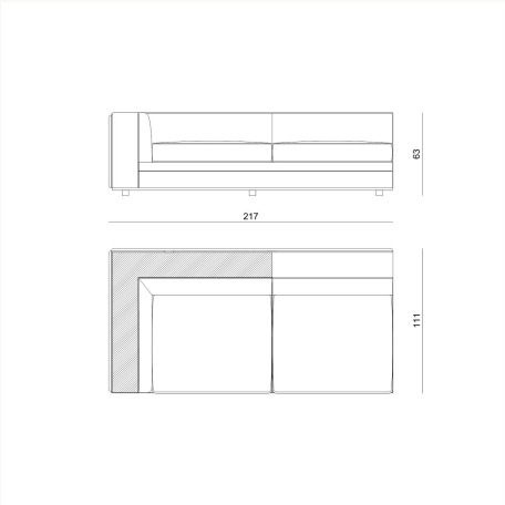
BYRK17 L 217 x H 64 x W 111 cm
