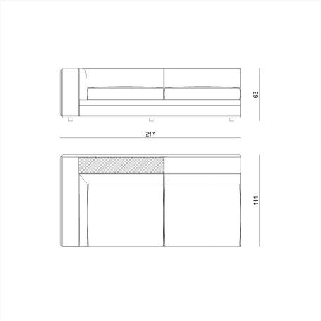
BYRK7F L 217 x H 64 x W 111 cm
