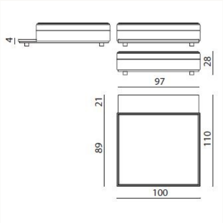
BABBTC L 100 x H 28 x W 110 cm
