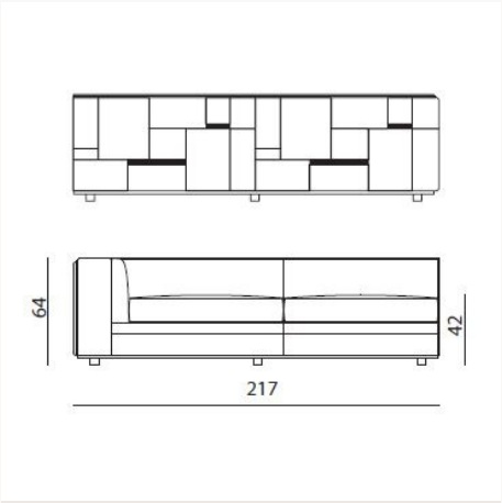
BABEL1 L 217 x H 64 x W 111 cm
