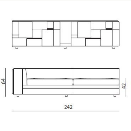
BABEL5 L 242 x H 64 x W 111 cm
