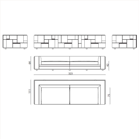
BABD32 L 323 x H 64 x W 111 cm
