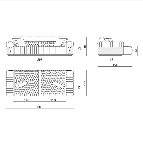
BBR24K L 300 x H 62 x W120 cm
