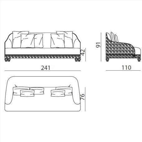
CTH240 L 240 x H 91 x W 110 cm
