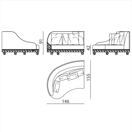
CTH4SC L 146 x H 91 x W 155 cm
