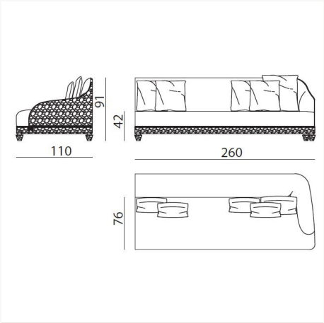
CTH26D L 260 x H 91 x W 110 cm
