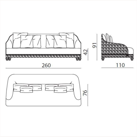
CTH260 L 260 x H 91 x W 110 cm
