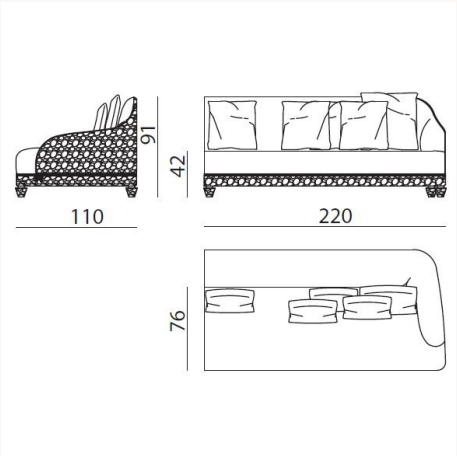
CTH22D L 220 x H 91 x W 110 cm
