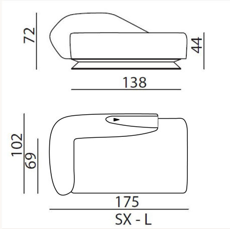
CTZ70S L 175 x H 72 x W102 cm
