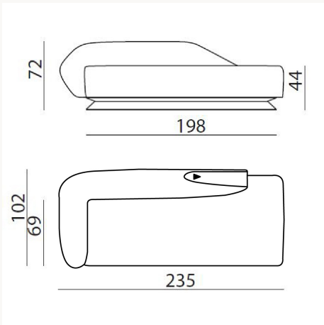
CTZALS L 235 x H 72 x W102 cm
