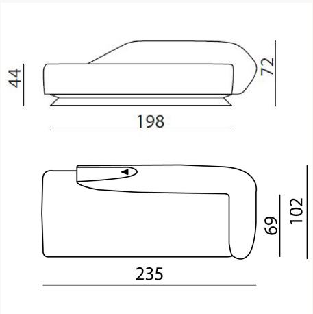
CTZA3D L 235 x H 72 x W102 cm
