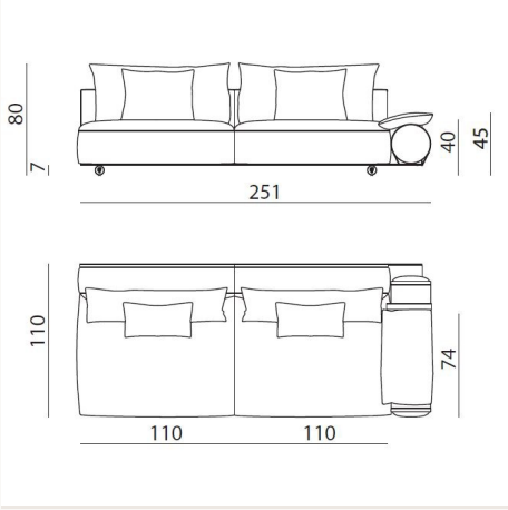
DLC SR8 L 251 x H 80 x W 110 cm
