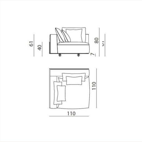
DLC SR5 L 110 x H 80 x W 110 cm
