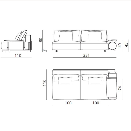
DLC SR1 L 231 x H 80 x W 110 cm
