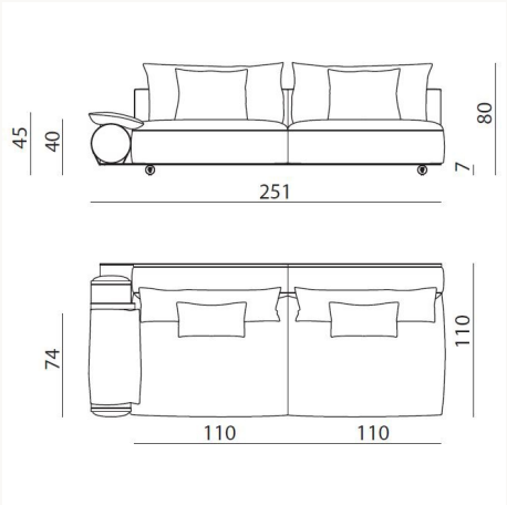
DLC SL8 L 251 x H 80 x W 110 cm
