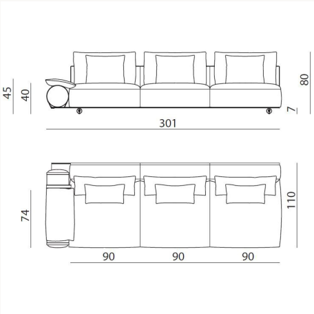
DLC SL9 L 301 x H 80 x W 110 cm
