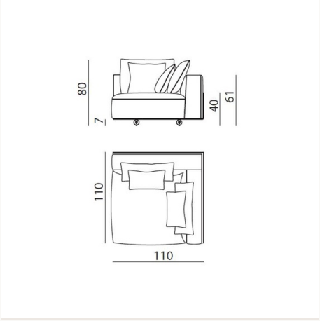
DLC SR6 L 110 x H 80 x W 110 cm
