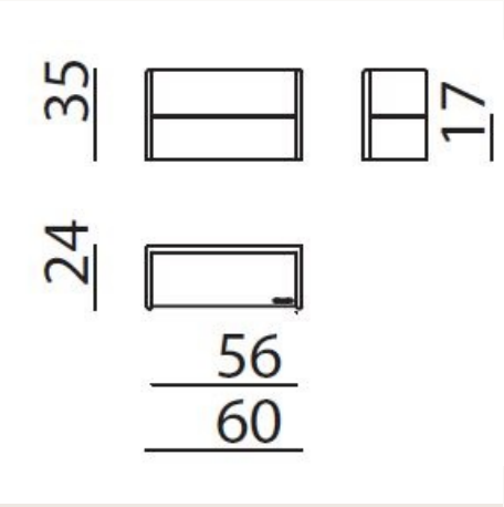
DS540P L 60 x H 35 x W 24 cm
