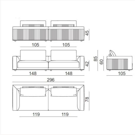
MLL296 L 296 x H 85 x W 105 cm
