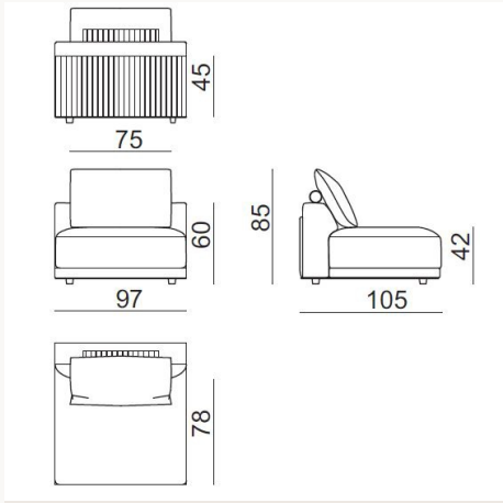
MLL97C L 97 x H 85 x W 105 cm
