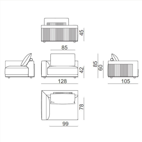
MLLE8S L 128 x H 85 x W 105 cm
