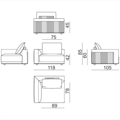
MLE1S L 118 x H 85 x W 105 cm
