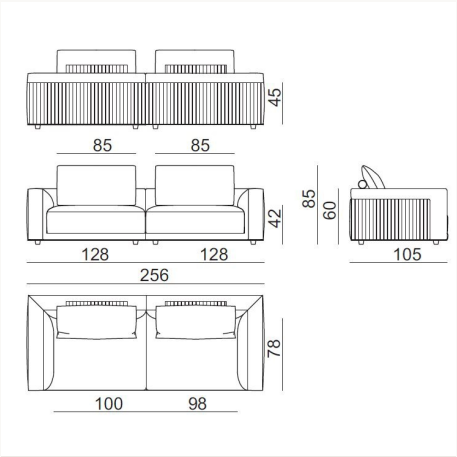
MLL256 L 256 x H 85 x W 105 cm
