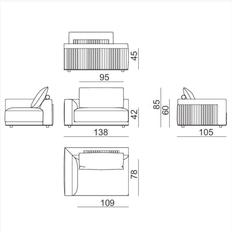
MLE3S L 138 x H 85 x W 105 cm
