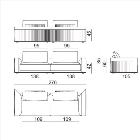
MLL276 L 276 x H 85 x W 105 cm
