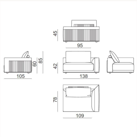
MLE3D L 138 x H 85 x W 105 cm
