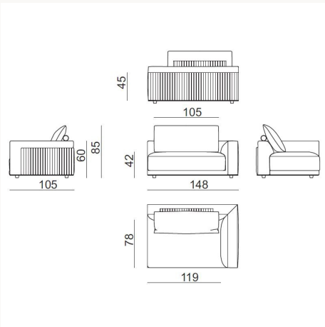
MLE4D L 148 x H 85 x W 105 cm
