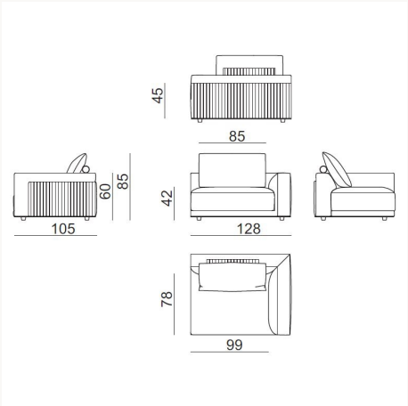
MLLE8D L 128 x H 85 x W 105 cm
