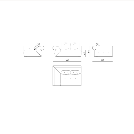
WLKW 45 L 162 x H 64 x W 116 cm
