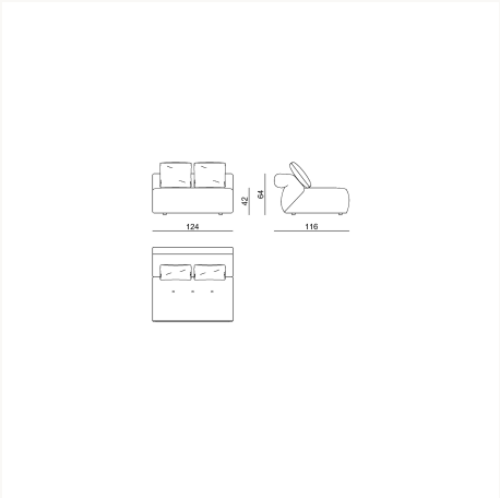
WLKW 53 L 124 x H 64 x W 116 cm
