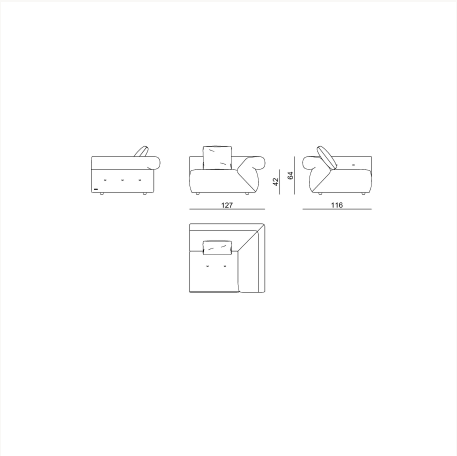
WLKW 52 L 127 x H 64 x W 116 cm
