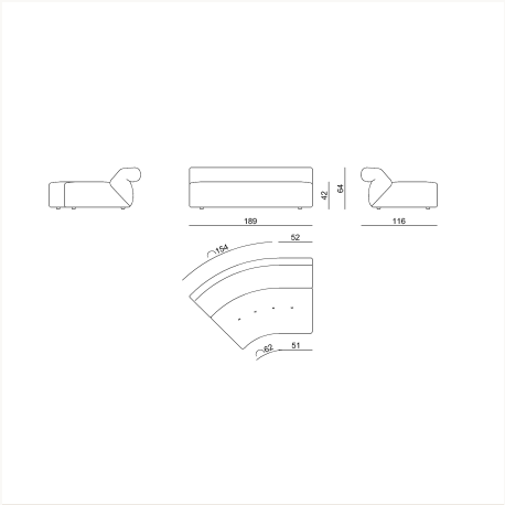
WLKW 60 L 189 x H 64 x W 116 cm
