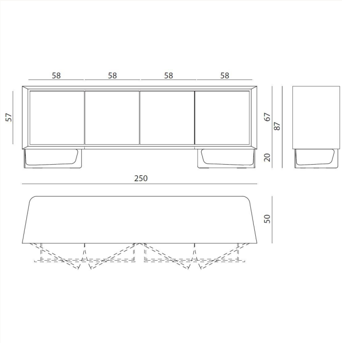
AZIM4D L 250 x H 87 x W 50 cm
