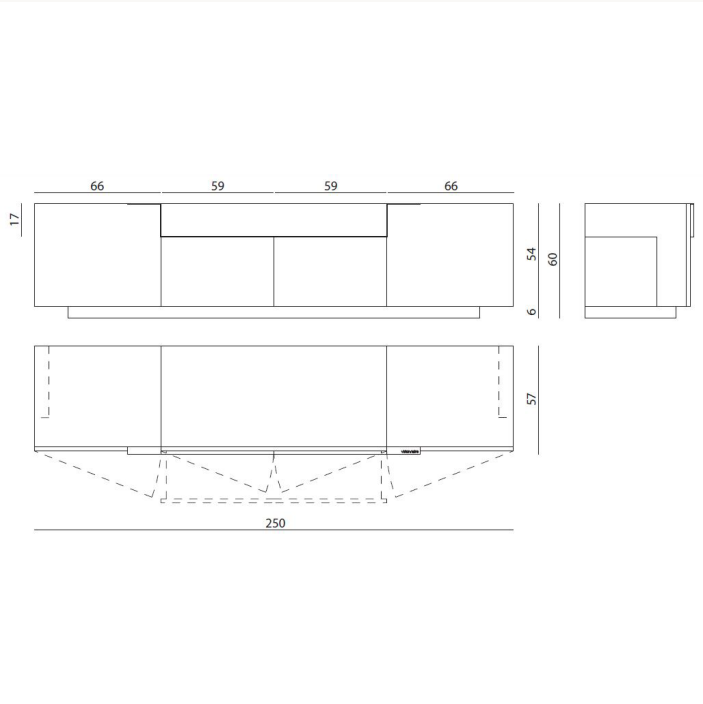
BRSBP6 L 250 x H 60 x W 57 cm
