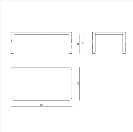
SRMKR9 L 220 x H 77 x W 120 cm
